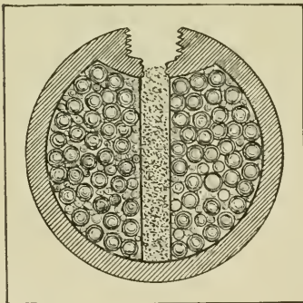
OLD STYLE SHRAPNEL.
